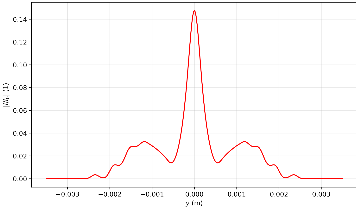
Intensity profile I(x=0, y, z=3.344)/I_0 , P_{in}=8.5P_{cr} , artificial time
